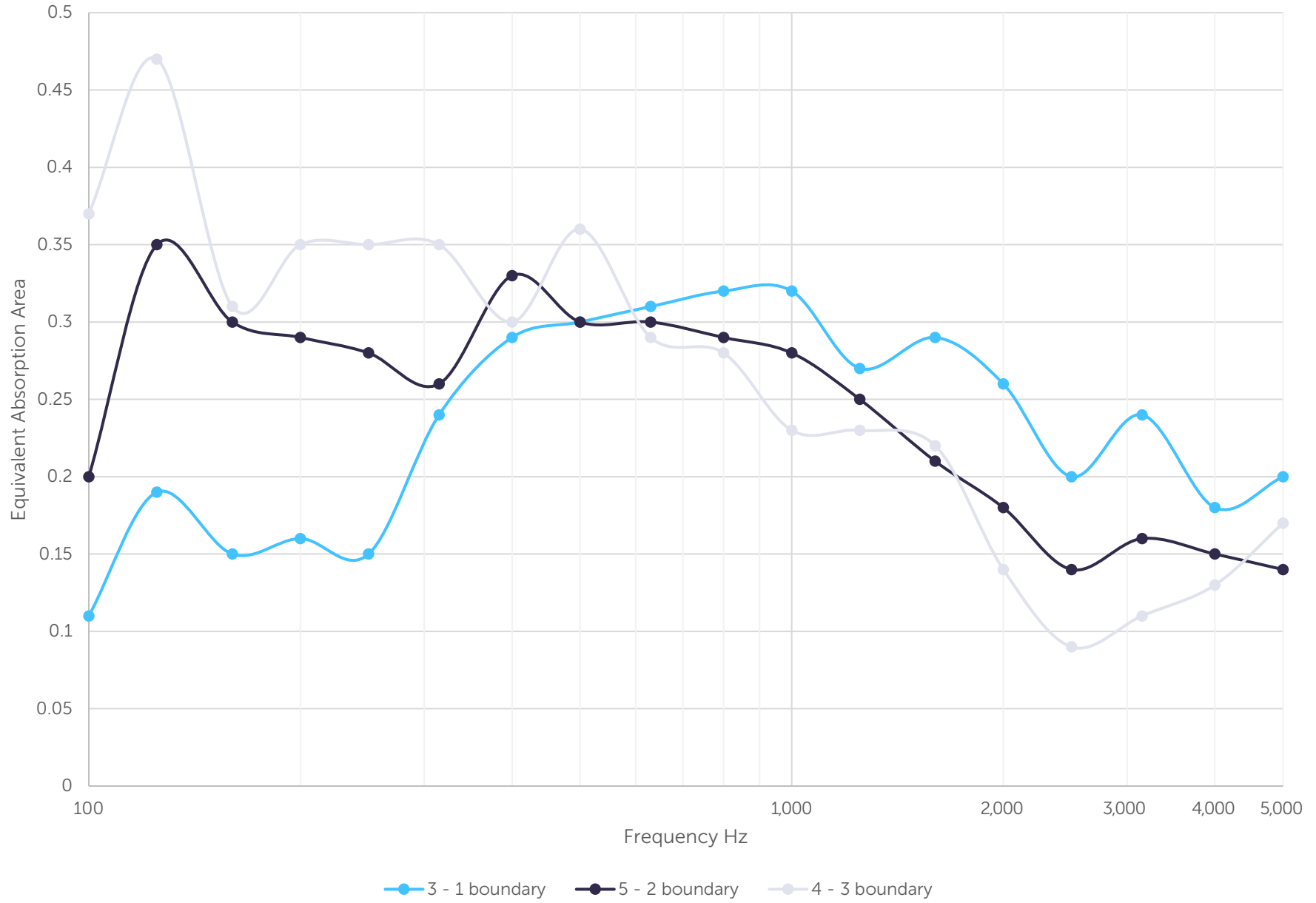
Equivalent Sound Absorption Area Per Object (Object Area = 0.36m 2 )
